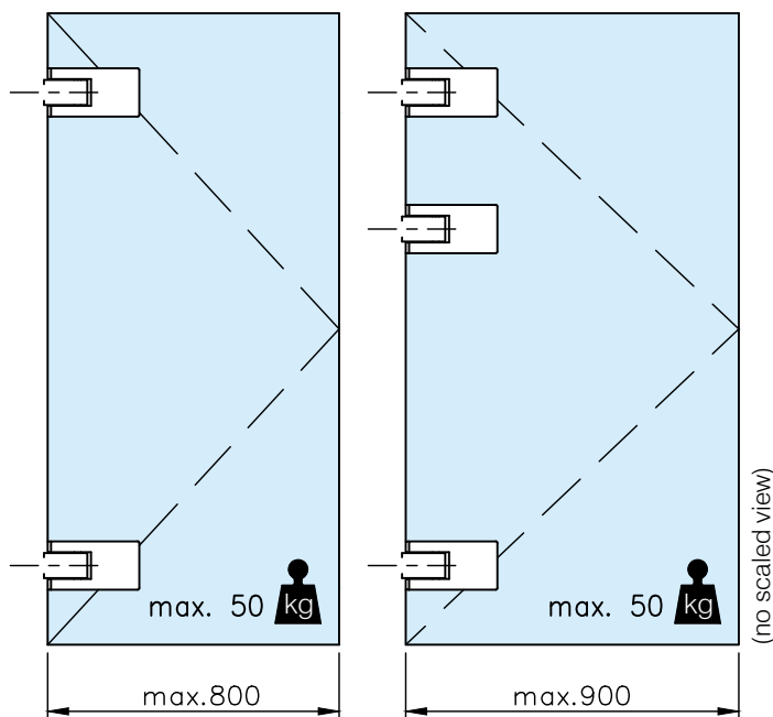
max. load weights and door width
